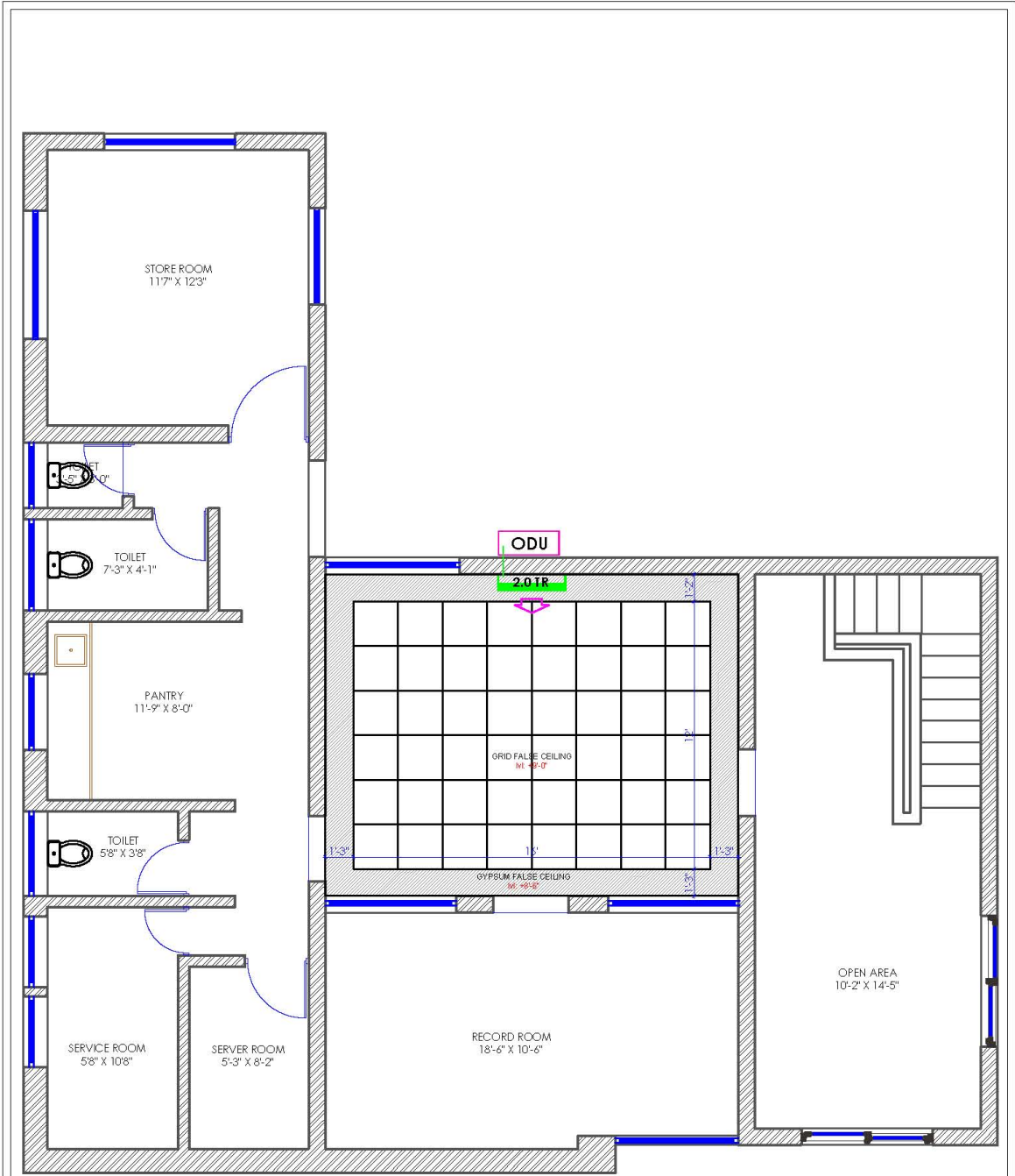
FIRST FLOOR FALSE CEILING PLAN
